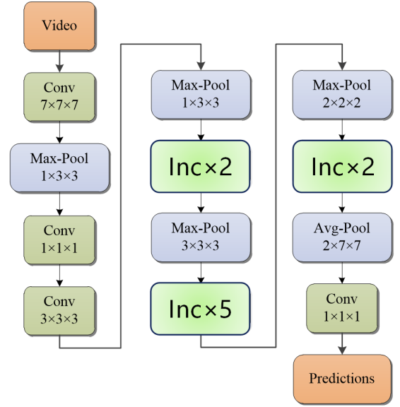
Figure 3. Schematic representation of the I3D network architecture.
