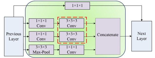
Figure 4. The inception module of I3D architecture.
